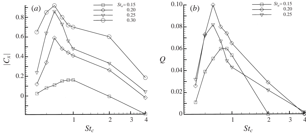
FIGURE 9. Thrust coefficient (a) and efficiency (b) as functions of St_c for a given St_a . Different St_a are represented by different symbols.
