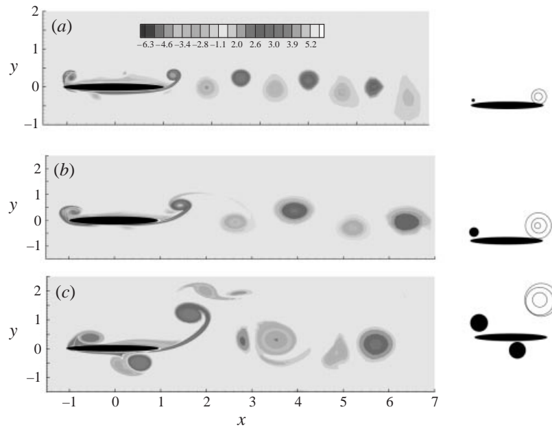
FIGURE 4. Contour plot of the wake vorticity at 1/8 th of a period for different frequencies: (a) f = 1.0 ( St_c = 2.0 ), (b) f = 0.5 ( St_c = 1.0 ), (c) f = 0.25 ( St_c = 0.5 ). The grey scale indicates the strength of the vorticity. Other parameters are: Re = 1000 and St_a = 0.16 . The sketches on the right-hand side summarize the basic structure of shed vortices. The leading- and trailing-edge vortices have different signs. In (a), the trailing-edge vortex is small and the leading-edge vortex is bound to the ellipse; in (b), the trailing-edge vortex is larger compared to (a) while the leading-edge vortex is still bound; in (c), both the leading- and trailing-edge vortices are shed (the vortex at the bottom of the ellipse is the leading-edge vortex shed in the previous cycle, which is best viewed in the animation of the simulation.) In the sketches, the black filled dots indicate clockwise-rotating vortices and the circles indicate counter-clockwise-rotating vortices.
