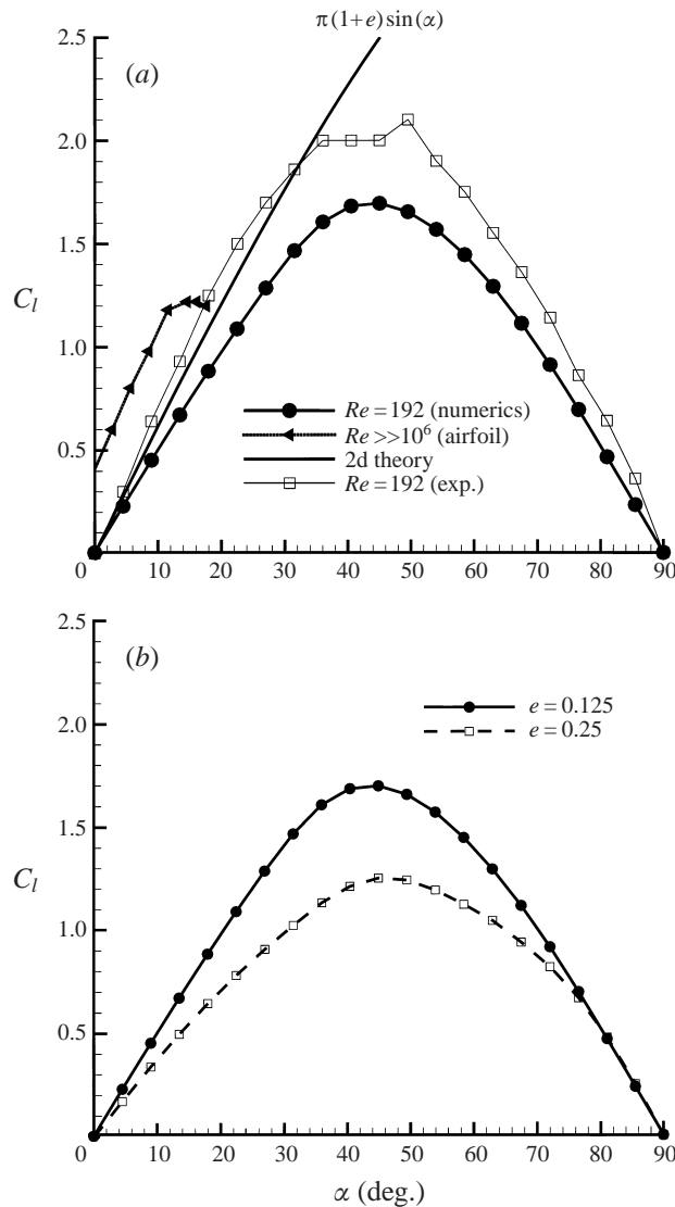
FIGURE 6. (a) Lift coefficient as a function of angle of attack. The experimental curve is taken from figure 4 in Dickinson & Götzt (1993). The data are measured at t_s = 2.0 . The classical curve for an airfoil curve is from Prandtl and Tietjens (1934). (b) Lift coefficient as a function of the thickness ratio of the ellipse.
