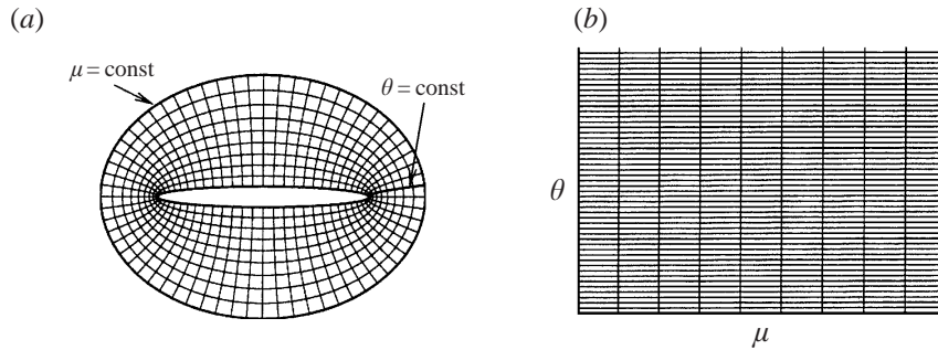
FIGURE 2. The elliptic coordinates (\mu, \theta) fitted to a two-dimensional wing. Confocal ellipses and hyperbolae correspond to constant \mu and \theta , respectively. The Cartesian coordinates, with periodic boundary conditions in the \theta -direction, conformally mapped from the elliptic coordinates.
